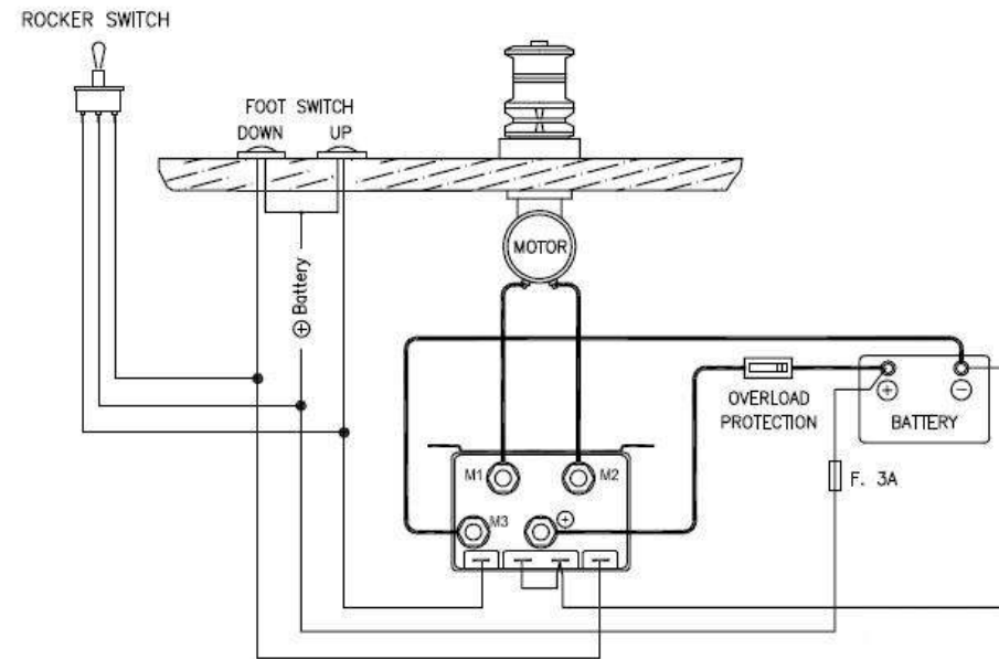
2 TERMINAL MOTORS
