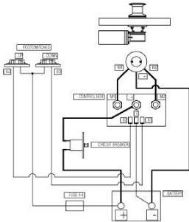
3 TERMINAL MOTORS
